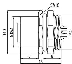
推荐开孔尺寸 Mounting hole - Through
