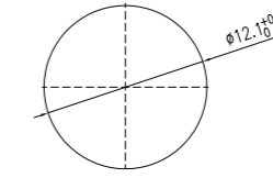
推荐开孔尺寸 Mounting hole - Through
