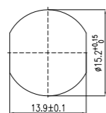
推荐开孔尺寸 Mounting hole - Through
